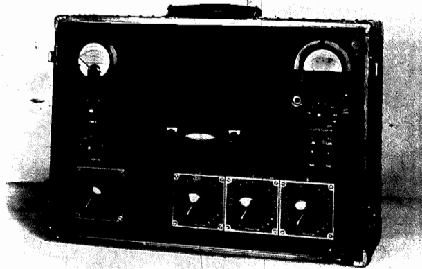
RCA VICTOR'S NEW OP-4 REMOTE PROGRAM AMPLIFIER
